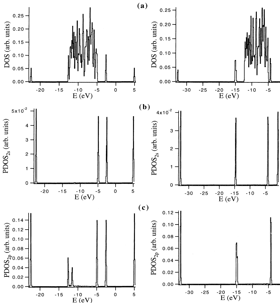
FIG. 7. Comparison between density of states of C (left column) and O (right column) adsorbed on the hollow site of Au 97 at (0,1.7,0.7) Å: (a) density of states, (b) 2 s projected density of states, and (c) 2 p projected density of states.
