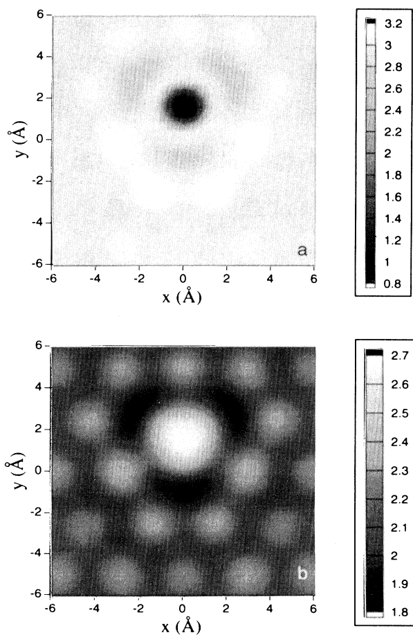
FIG. 8. Inversion of features from hole to protrusion as the tip-substrate separation increases, for a C atom adsorbed at the hollow site of Au_{97}(111) at (0,1.7,0.7) . The tip scans at (a) 3.5 Å and (b) 4 Å above the plane of Au atoms.
