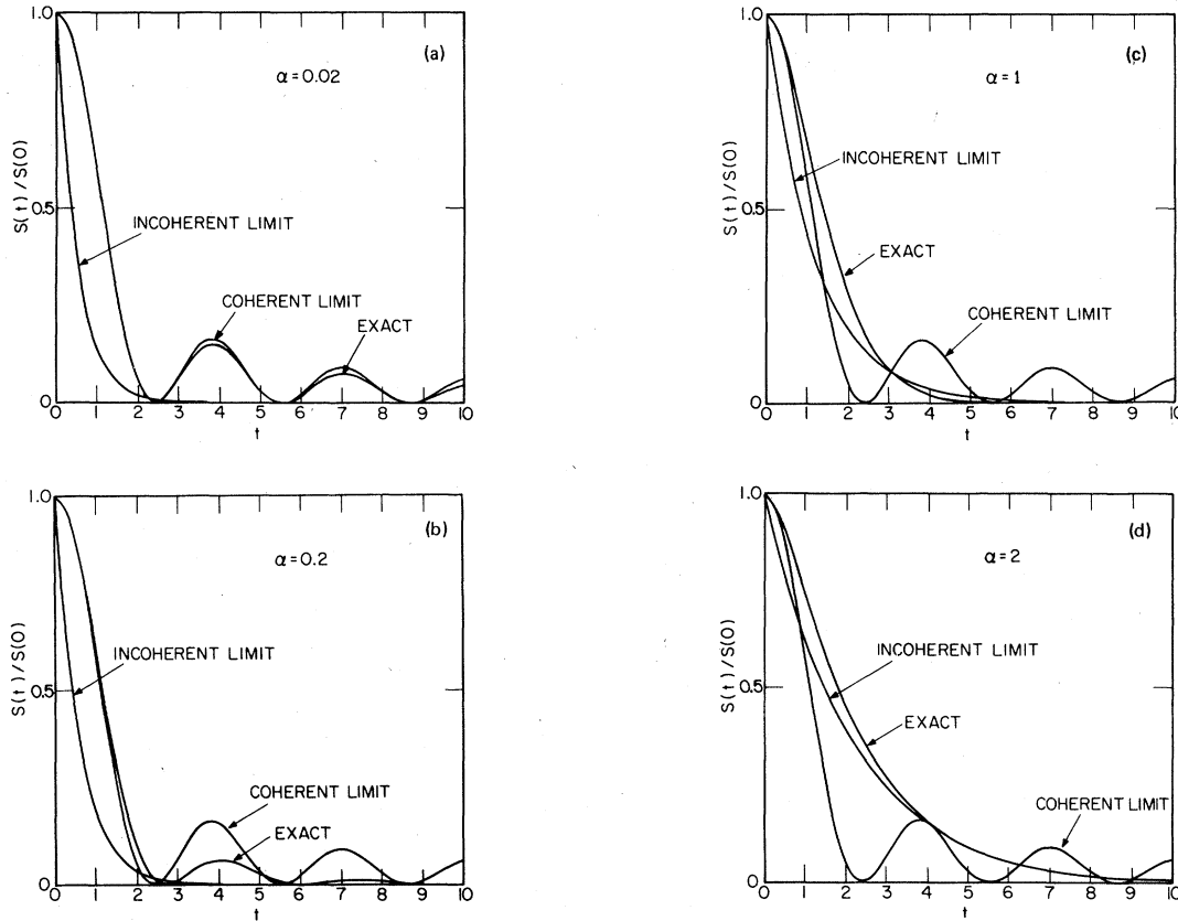
FIG. 1. Effect of coherence on the transient grating signal as a function of time. Curves respectively denote the signal in the incoherent limit given by (3.9), the coherent limit given by (3.10), and the intermediate exact expression given by (4.3). Parameters are arbitrary: 4J \sin(\Delta a/2) = 1 . The four cases correspond respectively to (a) \alpha = 0.02 , (b) \alpha = 0.2 , (c) \alpha = 1.0 , and (d) \alpha = 2.0 .
