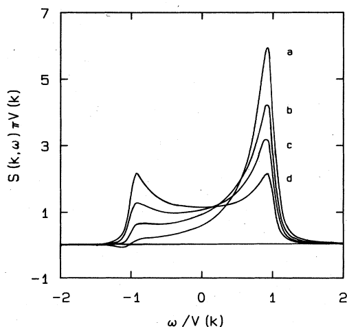
FIG. 2. Scattering function calculated directly from (2.1) and (3.7) for various temperatures. See text for discussion. Parameter values: curve a, k_B T = V ; curve b, k_B T = 2V ; curve c, k_B T = 4V ; curve d, k_B T = \infty . For all curves, \alpha/V(k)=0.1 , ka = \pi .
