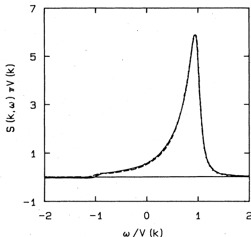
FIG. 3. Comparison of S(k, \omega) (—), S^s(k, \omega) (· · · ·), and S^a(k, \omega) (— — —) for k_B T = V , \alpha/V(k)=0.1 , ka = \pi . Both S^s(k, \omega) and S^a(k, \omega) possess the proper symmetries and are positive definite. The integrated intensities of S^s(k, \omega) and S(k, \omega) are each equal to the infinite temperature value, as required by the condition that I(k, 0) is independent of temperature.
