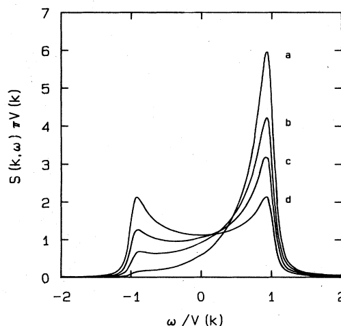
FIG. 4. Scattering function of Fig. 2 after the application of the symmetrization prescription (4.3). Parameter values: curve a, k_B T = V ; curve b, k_B T = 2V ; curve c, k_B T = 4V ; curve d, k_B T = \infty . For all curves \alpha/V(k)=0.1 , ka = \pi .
